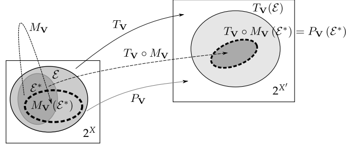
Figure 2: The relativity principle only implies that T_V \circ M_V(\mathcal{E}^*) = P_V(\mathcal{E}^*) . Covariance of \mathcal{E} would require that T_V(\mathcal{E}) = P_V(\mathcal{E}) , which is generally not the case, except if M_V : \mathcal{E}^* \rightarrow \mathcal{E} is surjective
